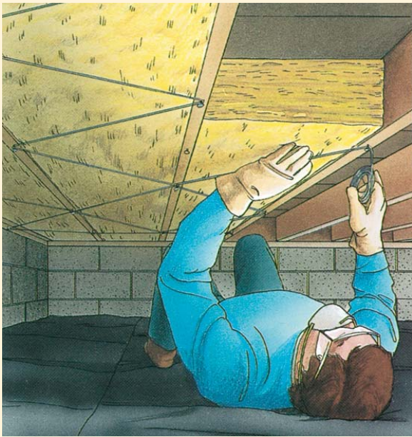
INSULATING CRAWLSPACES: Secure insulation between floor joists by stapling chicken wire or screening over the batts.
