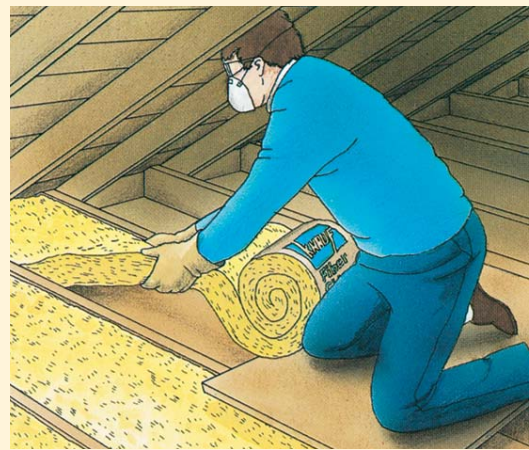
INSULATING WITH FACED INSULATION: Keep the vapor retarder down, toward the “warm-in-winter” area of your house.
