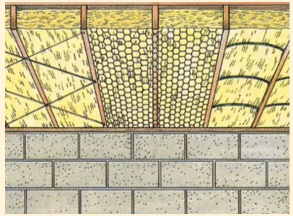
INSULATING CRAWLSPACES: Wire rods, chicken wire or screening can be used to secure insulation in crawlspaces.
